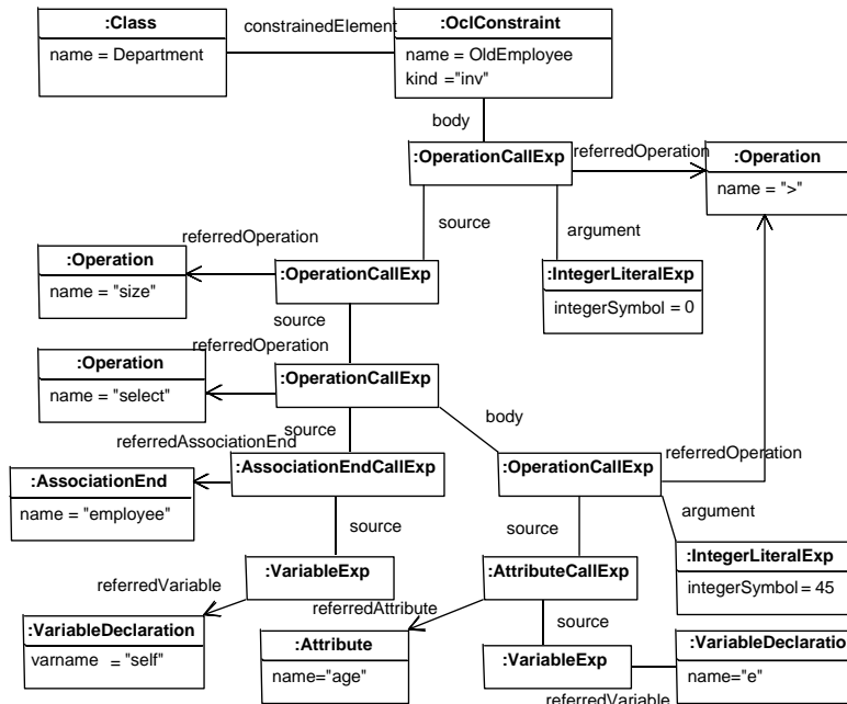
Figure 4.1 – Constraint OldEmployee as an instance of the OCL metamodel
