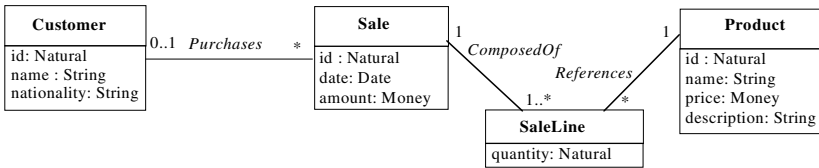
Fig. 2. The data model for the e-commerce application
